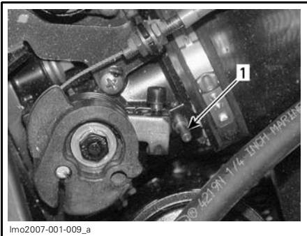
1. Raccord de lubrification
