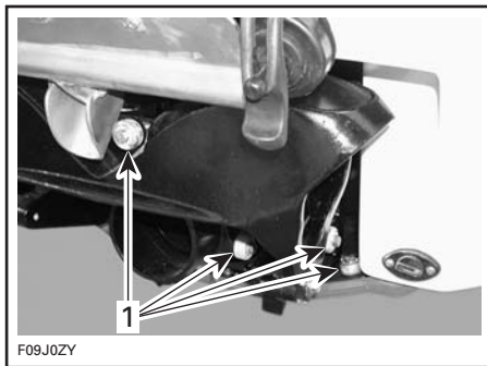
1. Anode installée
