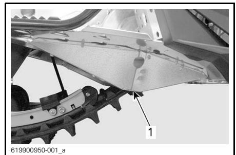
1. Drain plug access hole
