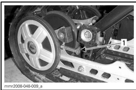
1. RH adjustment screw
