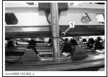
1. Deflection O-ring aligned with slider shoe
