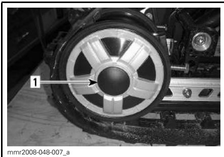
mmr2008-048-007_a 1. RH rear idler wheel cap
