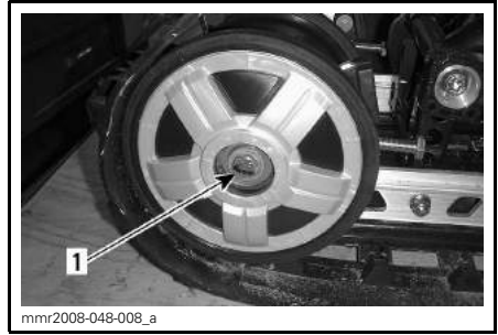
mmr2008-048-008_a 1. RH rear idler wheel bolt
