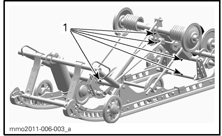
1. Grease fittings
