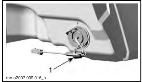
BEHIND AIR INTAKE SILENCER 1. Fuse location
