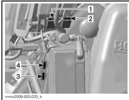
RH SIDE OF ENGINE COMPARTMENT 1. 15 A headlight fuse (RED/ORANGE wire) 2. 20 A accessories fuse (RED/YELLOW wire) 3. 30 A charging system fuse 4. 5 A ECM (Engine Control Module) fuse
