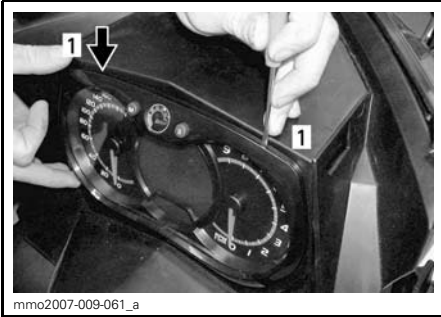
TYPICAL 1. Locking tab
