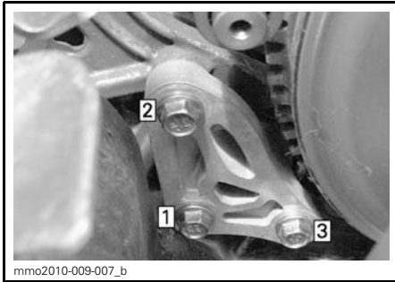
TIGHTENING SEQUENCE
