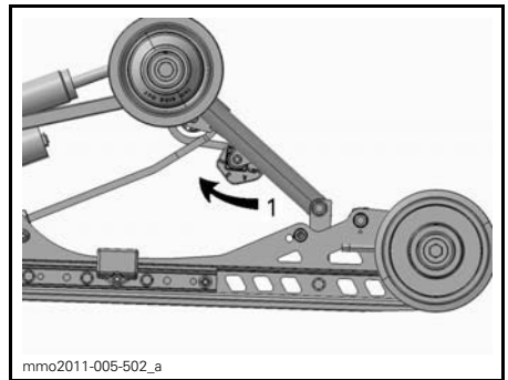
TYPICAL - rMOTION RACING - LH SIDE 1. Adjust spring preload
