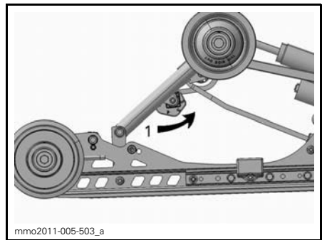
TYPICAL - rMOTION RACING - RH SIDE 1. Adjust spring preload
