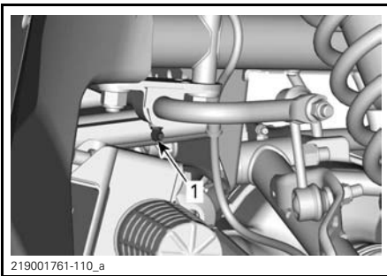
219001761-110_a TYPICAL - FRONT STABILIZER BAR 1. Grease fitting
