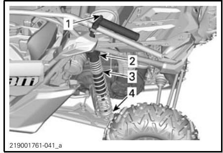
TYPICAL - MAVERICK XRS AND XRC TURBO R MODELS - REAR SUSPENSION
