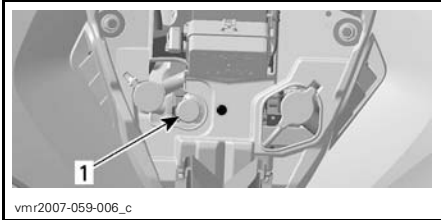
1. Coolant reservoir
