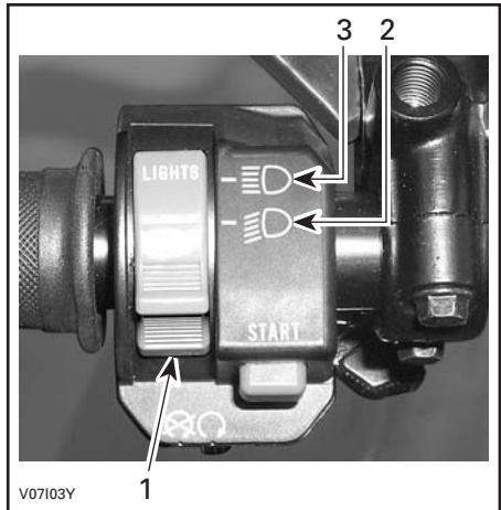
HEADLAMP SWITCH FUNCTIONS
