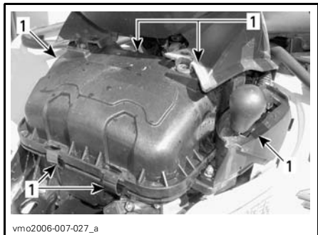
1. Release clamps
