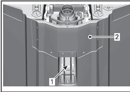
1. 犠牲陽極
