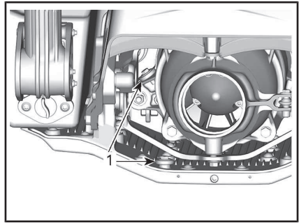
1. 犠牲陽極
