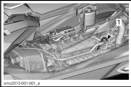
1. Cross over-slang
