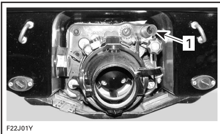
1. Spoelkoppeling
