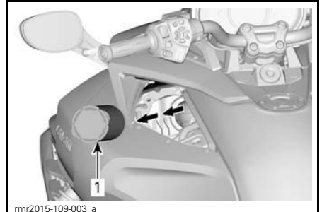
TYPICAL - REMOVE AIR FILTER FROM AIR INTAKE SILENCER. 1. Air filter
