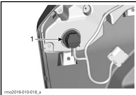
1. Turn bulb holder clockwise to release it
