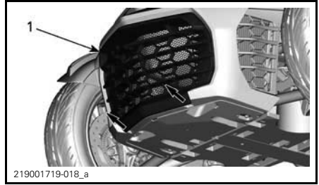
1. Front grille
