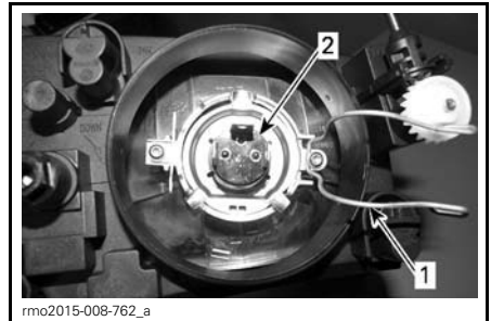
1. Bulb retaining spring 2. Bulb housing
