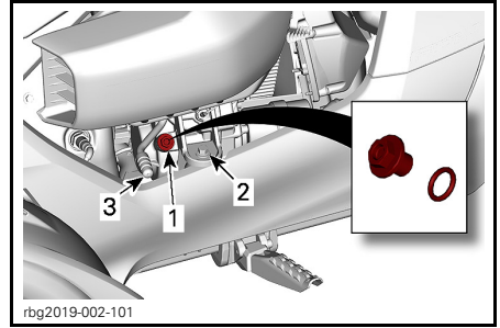
GEARBOX OIL FILLER PLUG LOCATION
