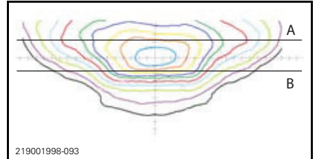
TYPICAL - HEADLIGHT REFLECTION ON TEST SURFACE
