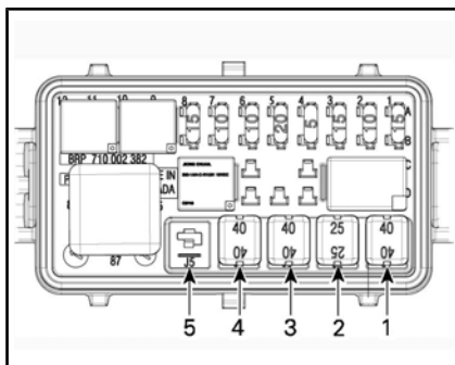
JCASE-SULAKKEET – VASEN SULAKEKOTELO
