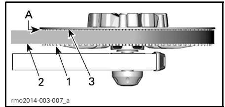
REAR SPROCKET 1. Rear sprocket teeth 2. Belt 3. Sprocket internal flange A. GAP "Y"
