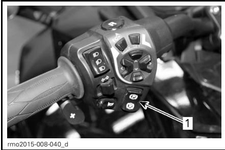
1. Parking brake switch
