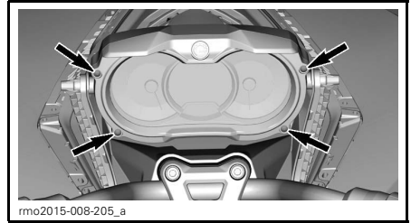
RETAINING SCREWS TO REMOVE
