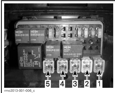
JCASE FUSES - LEFT FUSE BOX
