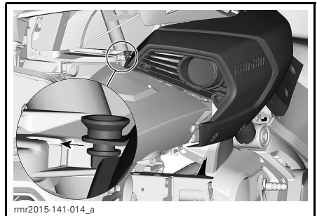
ALIGNING PANELS PROPERLY
