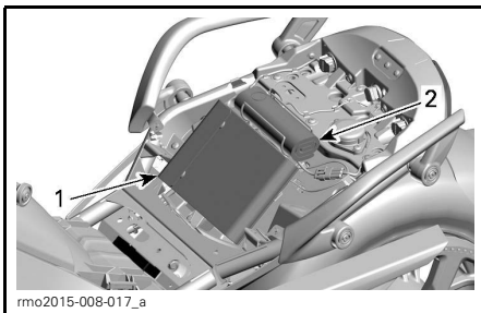
LIFTING PASSENGER SEAT TO REMOVE IT
