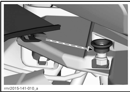
ALIGNING TABS IN CORRECT INSTALLATION LOCATION
