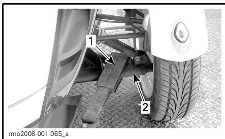
TYPICAL 1. Strap 2. Lower suspension arm
