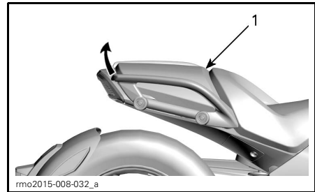
LIFTING PASSENGER SEAT TO REMOVE IT
