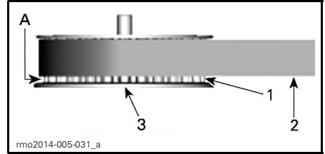
FRONT SPROCKET 1. Front sprocket teeth 2. Belt 3. Sprocket internal flange A. GAP "X"
