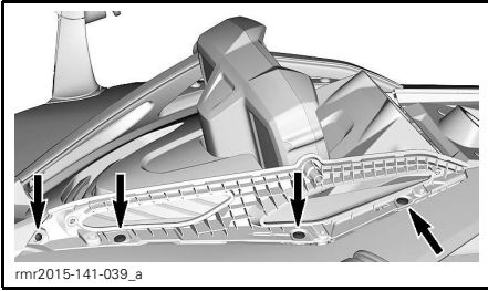
RETAINING SCREWS TO REMOVE
