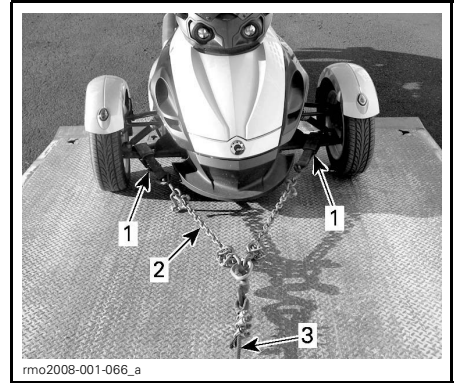
TYPICAL 1. Strap around front suspension lower arms 2. Chains to avoid damaging the bumper cover 3. Winch cable
