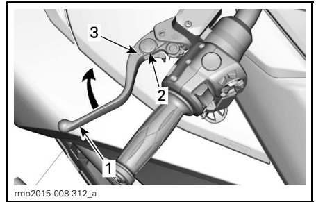
TYPICAL - CLUTCH LEVER ADJUSTMENT
