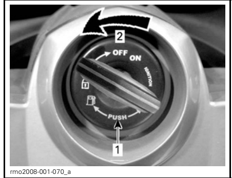
KEY POSITION TO OPEN FRONT STORAGE COMPARTMENT
