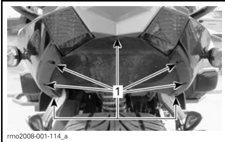
WHEEL WELL PANEL 1. 7 Torx screws location
