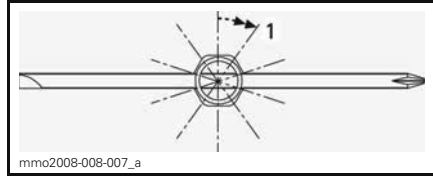
USED SPARK PLUG 1. Tighten 1/10 of a turn
