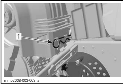
1. Retaining pin
