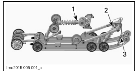
PPS-5900A AFTURFJÖÐRUN
