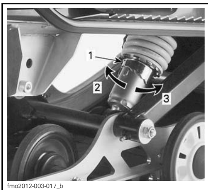
TYPICAL - FRONT SUSPENSION 1. Front springs for handling
