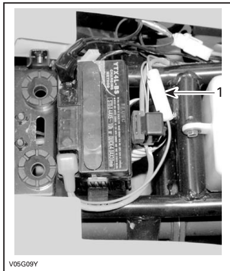
1. Fuse holder
