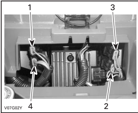
1. Fuse holders
