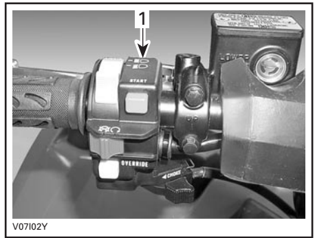
TYPICAL 1. Multi-function switch
