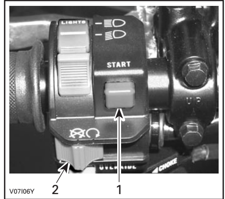
V07106Y TYPICAL 1. Start button 2. Engine stop switch
