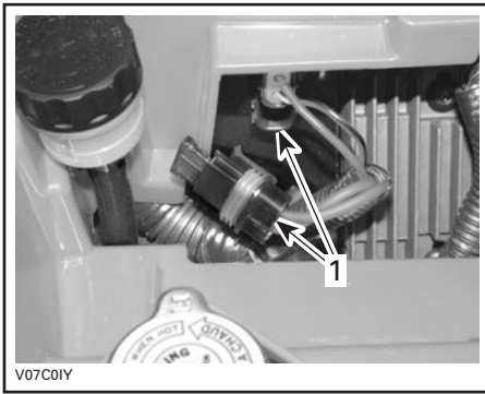
1. Fuse holders
