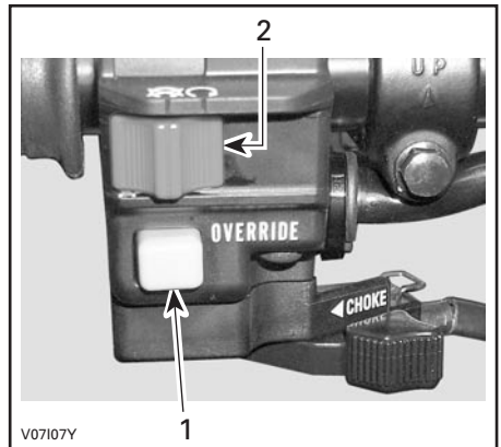
V07107Y TYPICAL 1. Override button 2. Engine stop switch
