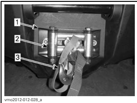
1. Winch 2. Roller fairlead 3. Winch hook
