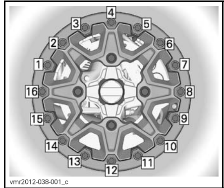
vmr2012-038-001_c FINAL TIGHTENING SEQUENCE
