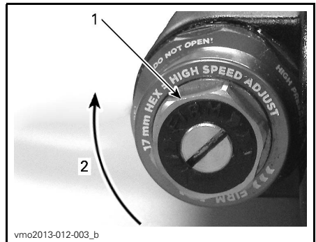
1. High speed compression damping adjuster 2. Firmer
