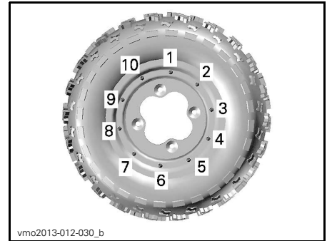
10-BOLT BEADLOCK WHEELS — FINAL STEP TIGHTENING SEQUENCE
