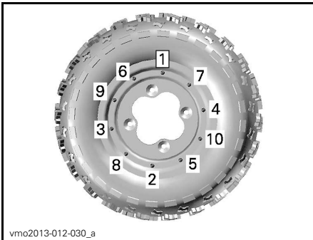
10-BOLT BEADLOCK WHEELS — FIRST AND SECOND STEPS TIGHTENING SEQUENCE
