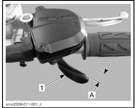
1. Throttle lever A. 2 to 4 mm (5/64 to 5/32 in)
