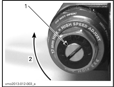
1. Low speed compression damping adjuster 2. Firmer
