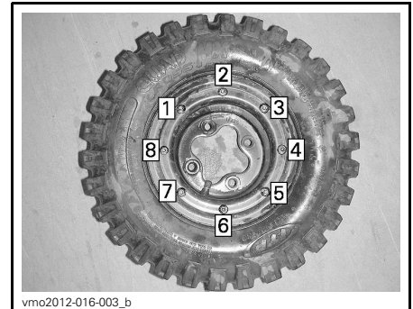
8-BOLT BEADLOCK WHEELS — FINAL STEP TIGHTENING SEQUENCE
