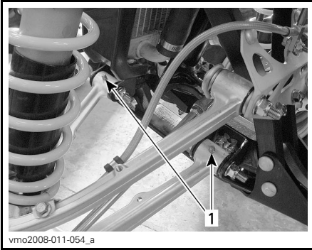
TYPICAL — LOWER SUSPENSION ARM 1. Grease fittings
