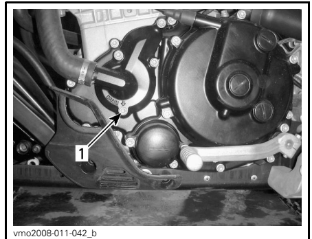
LH SIDE OF ENGINE 1. Coolant drain plug
