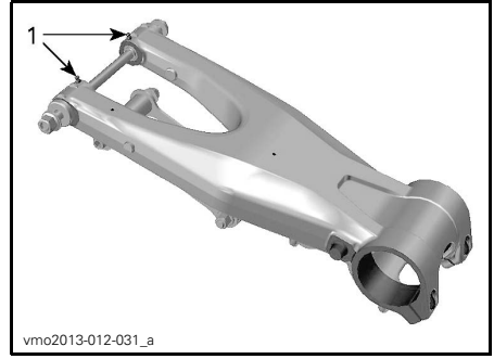
FRONT PIVOT ARM 1. Grease fittings
