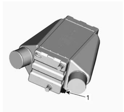
1. 犠牲陽極
