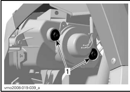
1. Adjustment screws
