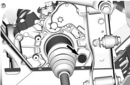
FRÄMRE SMART-LOK-DIFFERENTIAL
