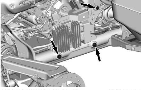
VOLTAGE/REGULATOR SCREWS SUPPORT SCREWS
