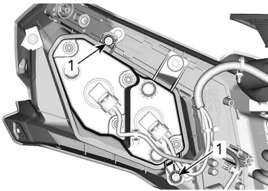
1. Adjustment screws
