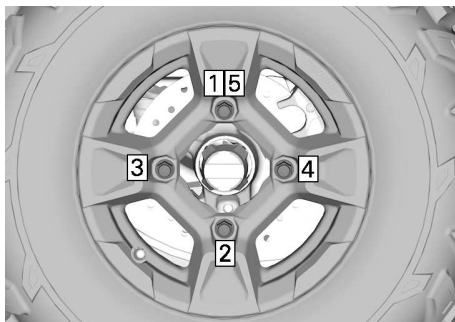
TIGHTENING SEQUENCE
