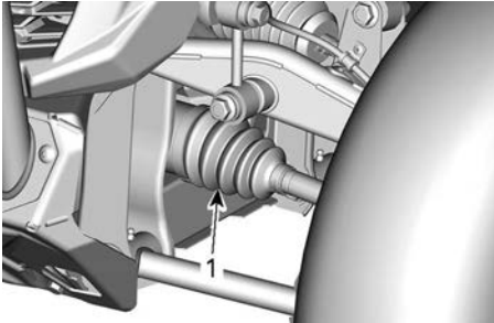
TYPBILD — FRAMDIFFERENTIALSIDA
