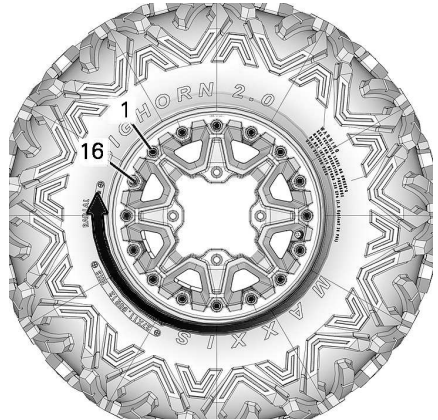
TYPICAL - FINAL TIGHTENING SEQUENCE
