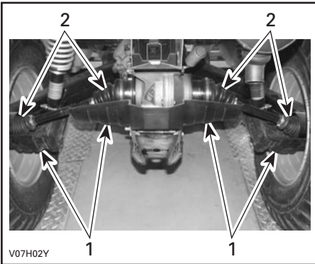
ALL MODELS — REAR OF VEHICLE
