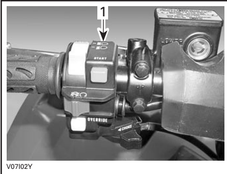
1. Multi-function switch
