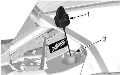
1. Oil dipstick 2. Oil filler tube
