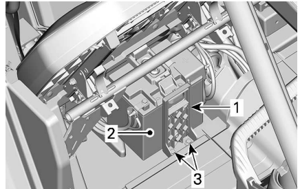
1. Battery holder 2. Battery 3. Battery holder retaining screw(s)
