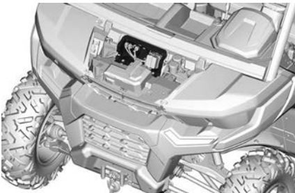
SULAKEKOTELON TUKI
